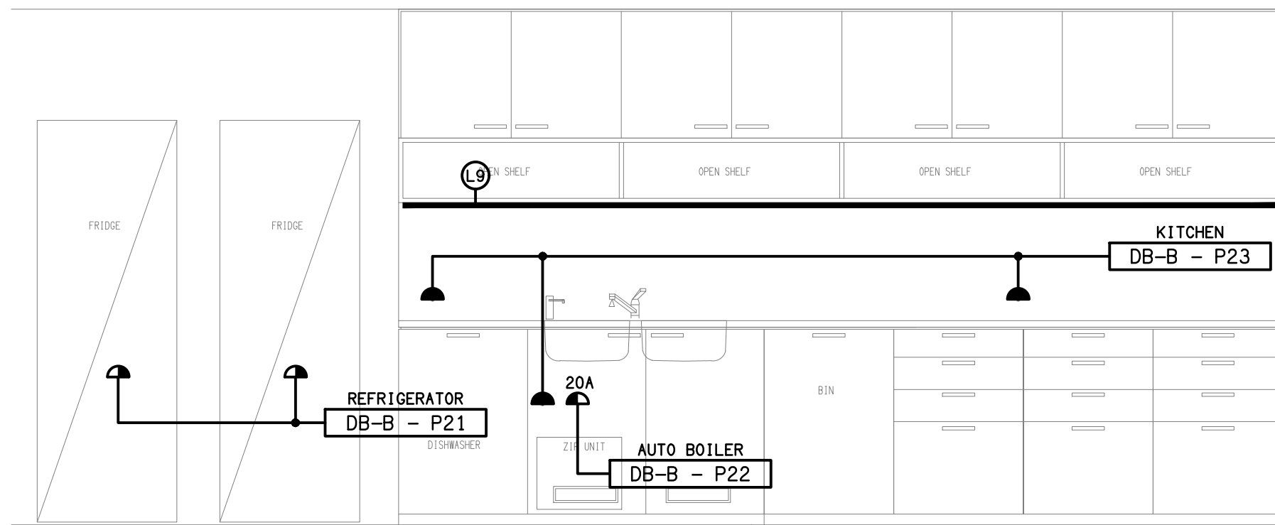
DETAIL B MEETING KITCHENETTE ELEVATION SCALE 1: 25
