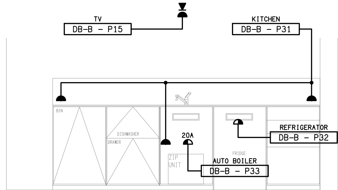
DETAIL A CUSTOMER KITCHENETTE ELEVATION SCALE 1: 25
